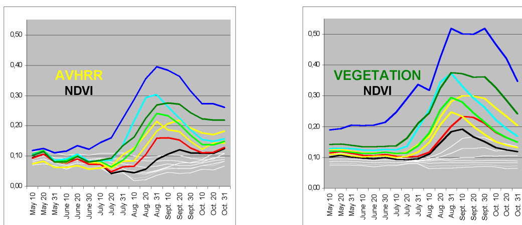
Figure 4 : Comparison of profiles from multitemporal classification of NDVI (MVC on decade) using NOAA-AVHRR and VEGETATION data from May to October 1999.
