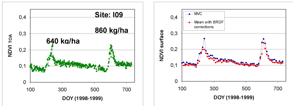
Figure 7 : Daily and decade temporal profile with VEGETATION data in 1998 and 1999 and differences observed between two methods of compositing MVC and mean with BRDF and atmospherical corrections.
