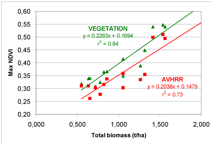
Figure 2 : Comparison of biomass estimation using NOAA-AVHRR and VEGETATION data (Niger sites, 1999).
