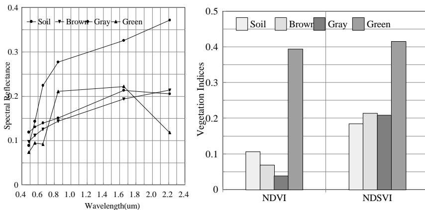
Figure 6 : Spectral responses and vegetation indices of soil, green, senescent, and gray vegetation.
