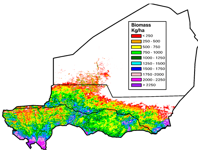
Figure 8 : Niger VEGETATION biomass map (kg/ha) derived from NDVI, May to October 1999.
