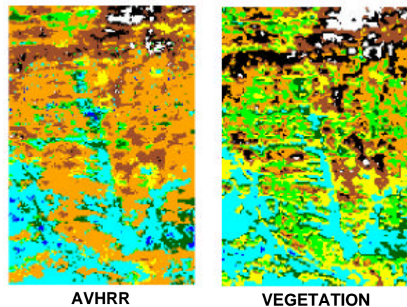
Figure 3 : Comparison of multitemporal classification using NOAA-AVHRR and VEGETATION data (1999).
