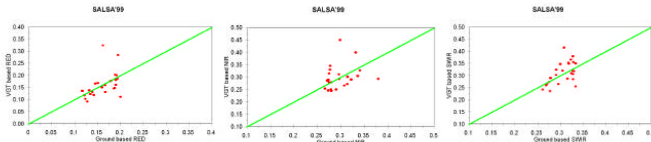
Figure 1 : Comparison between ground based and VEGETATION based reflectances corrected for atmosphere, view and sun angle effects.
