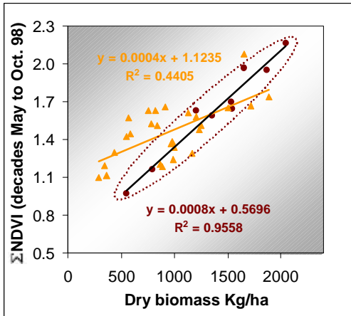
Figure 5 : Empirical relationship between integrated VEGETATION NDVI and total biomass in Niger in 1998. The fitted regression drawn in black corresponds to dark soils (clay) situated on plains and valleys.
